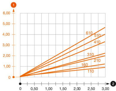
Load diagram, bracket type AS 30
